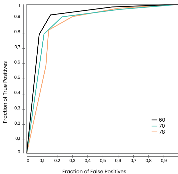
Receiver Operating Characteristic (ROC) Curves for Different Tube Voltages (60, 70, 78 kV)
