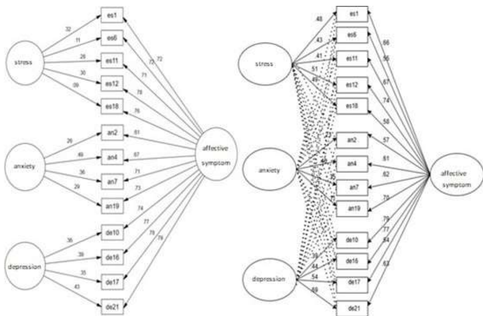
Figure 4 Graphic representation of the confirmatory bifactorial (left) and semi-confirmatory (right) DASS-13 measurement model
