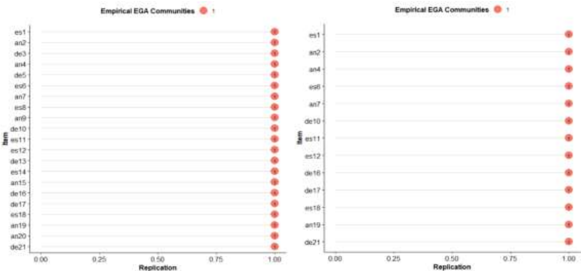
Figure 2 Stability of the questionnaire items
